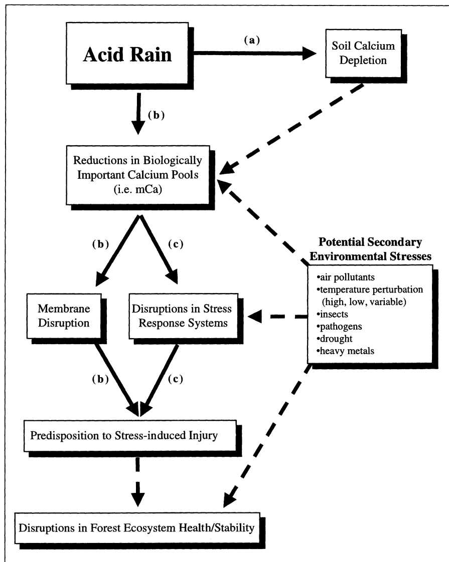
Figure 9. The impacts of acid deposition on ecosystem calcium nutrition, health, and sustainability. Known impacts are indicated by solid lines, and potential impacts are indicated by dashed lines. Letters indicate references for the known components: a, Lawrence et al. (1995), Likens et al. (1996); b, Schaberg and DeHayes (in press), Schaberg et al. (in press b); c, Dhindsa et al. (1993), Monroy et al. (1993), Sheen (1996).
