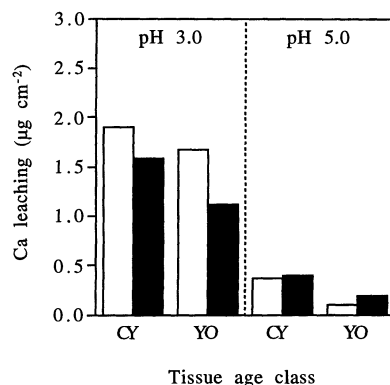
Figure 5. Influence of pH 3.0 and pH 5.0 mists on in vitro calcium leaching of needles of red spruce seedlings. CY, current-year needles; YO, year-old needles; open bars, needles plus twigs; solid bars, needles alone (Schaberg and DeHayes in press).
